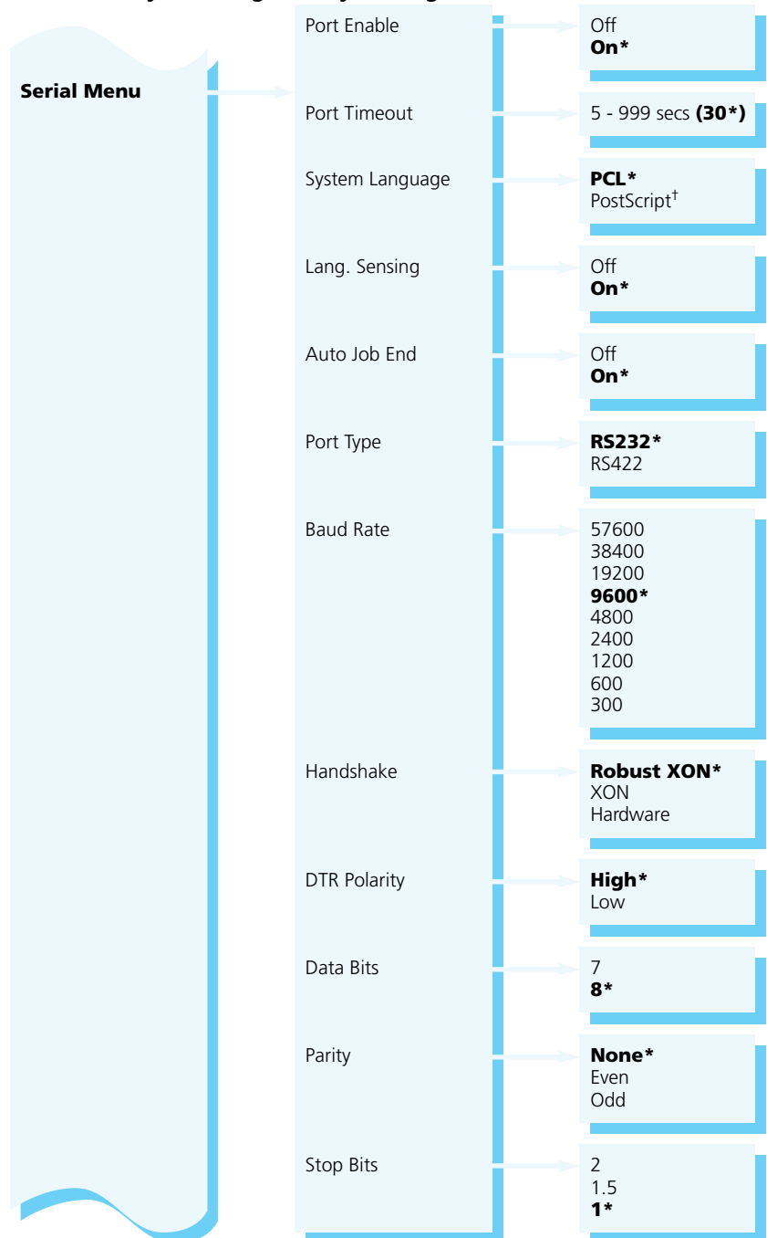
Figure 3.13 Interface Menu hierarchy showing factory settings (continued)
